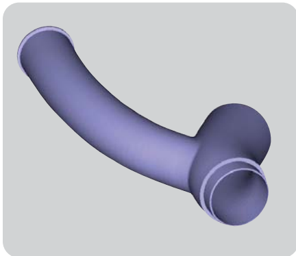
Image 1: Bell Helicopter's Xworx prototyping lab used FDM to build functional models of communication-wiring conduit for the Osprey. Images 2 and 3: Two conduit sections installed for ground testing.
